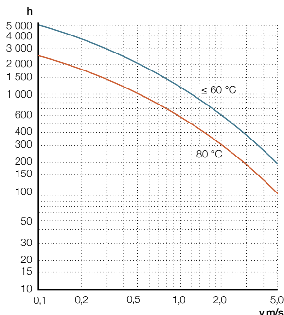
Relubrication interval
