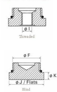
Shape A - Seal in angle
