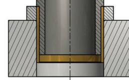
Installation with a force fitting mandrel and a guide bush (advised for bushings with ID over \phi 80\text{mm} )
