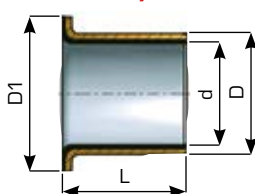
TEF-MET®/B Flange bushing
