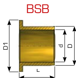
BRO-MAS® Flange bushing
