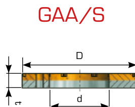
GAP-MET®/S Thrust washer
