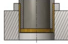
Installation with a force fitting mandrel and a guide bush (advised for bushings with ID over ø80mm)
