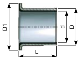
TEF-MET® Flange bushing
