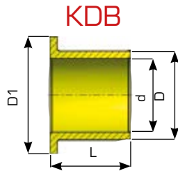
COM-KU®/D Flange bushing
