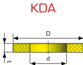
COM-KU®/D Thrust washer
