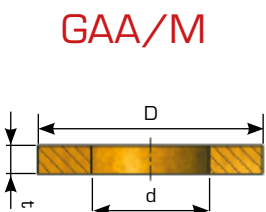
GAP-MET®/M Thrust washer
