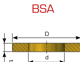
BRO-MAS® Thrust washer
