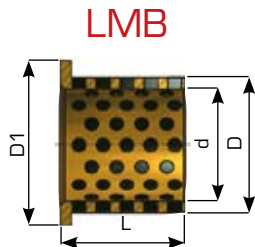
LUB-MET® Flange bushing
