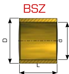
BRO-MAS® Cylindrical bushing
