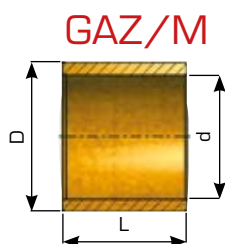
GAP-MET®/M Cylindrical bushing
