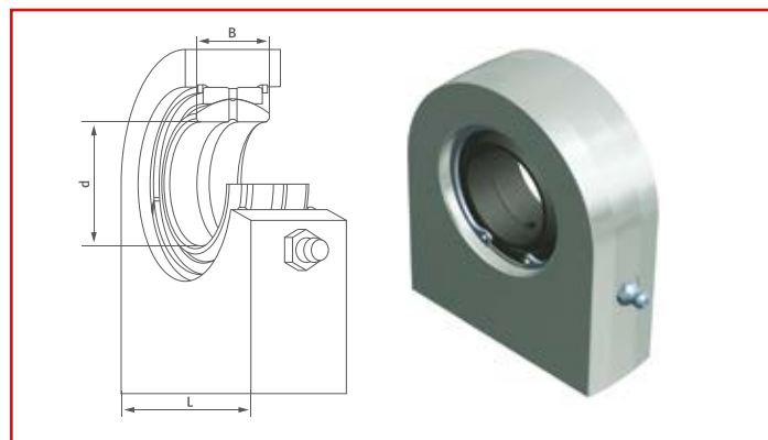
Hydraulic rod end, steel / steel with angular weld-on bolt
