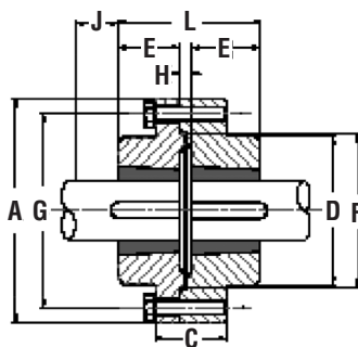
Coupling Assembly HF
