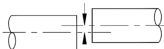
PARALLEL MISALIGNMENT - Shafts are in line angularly and parallel to each other, but are off-set.
