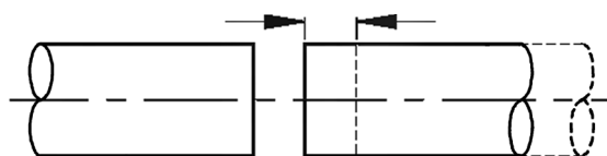
AXIAL MISALIGNMENT - includes applicable 'end float' - shafts move axially increasing or decreasing the distance between shaft ends.
