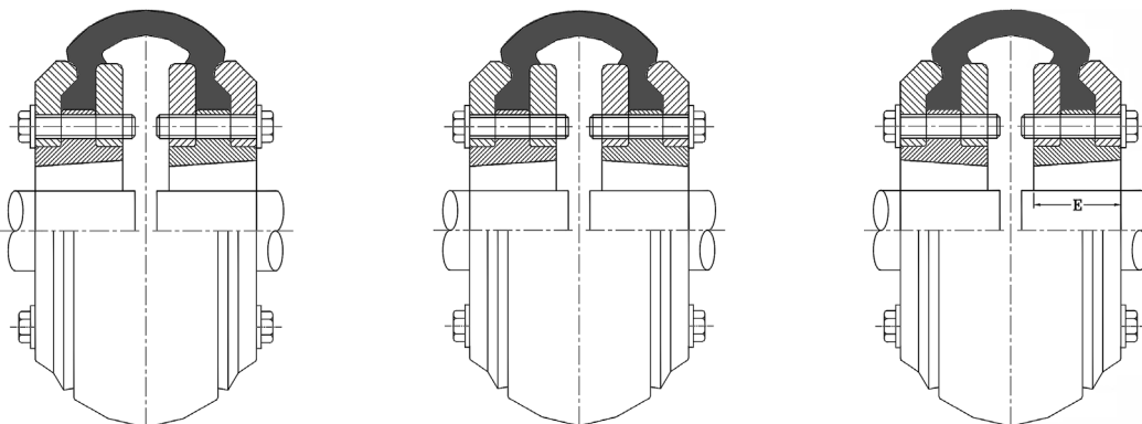
SIZES F70-120 (Reversible)
