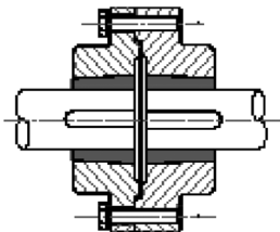
Coupling Assembly FF
